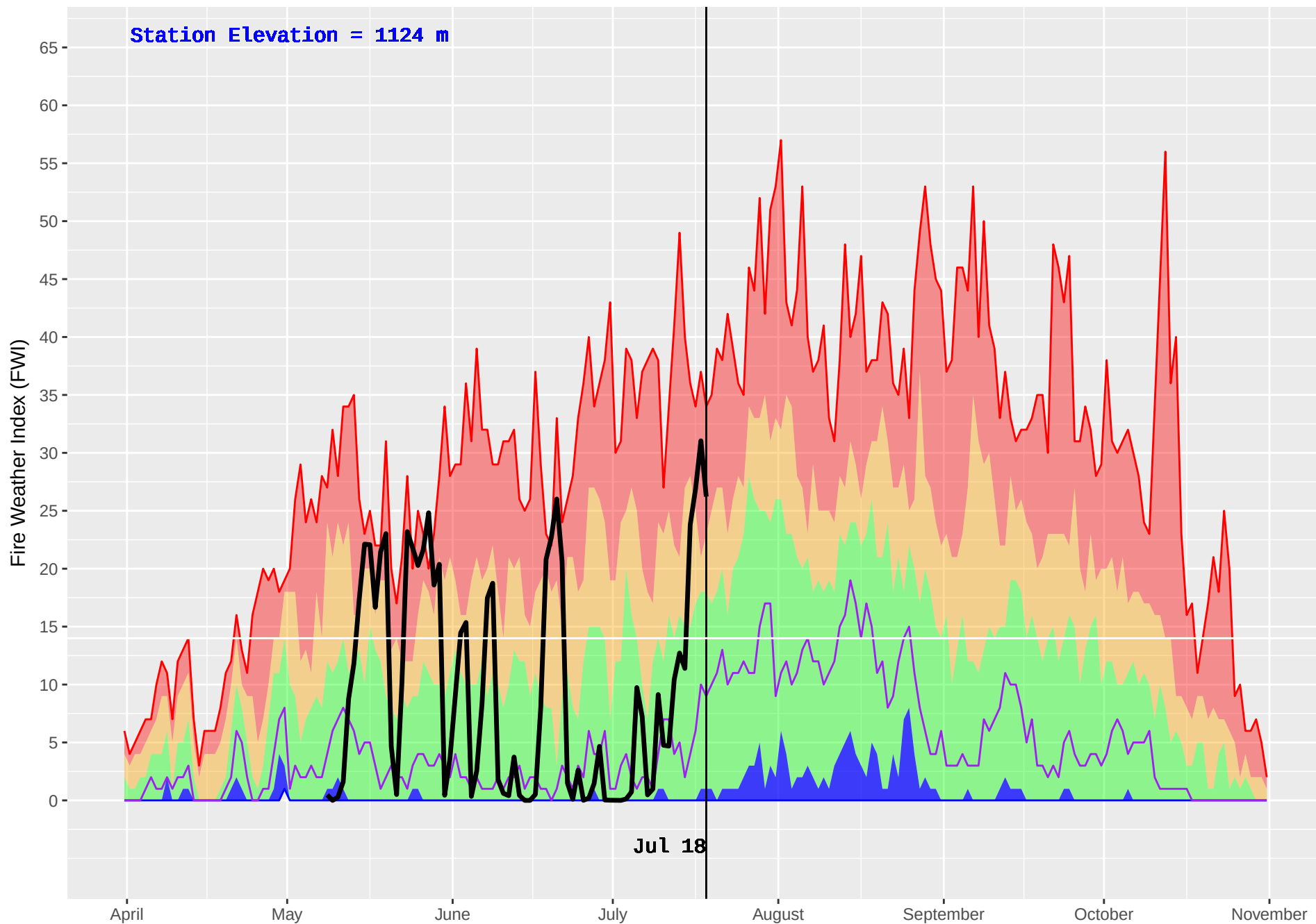
COLDSCAUR LAKE (232) : Historical (1979–2016) and Current (2018) Daily Fire Weather Index (FWI)
