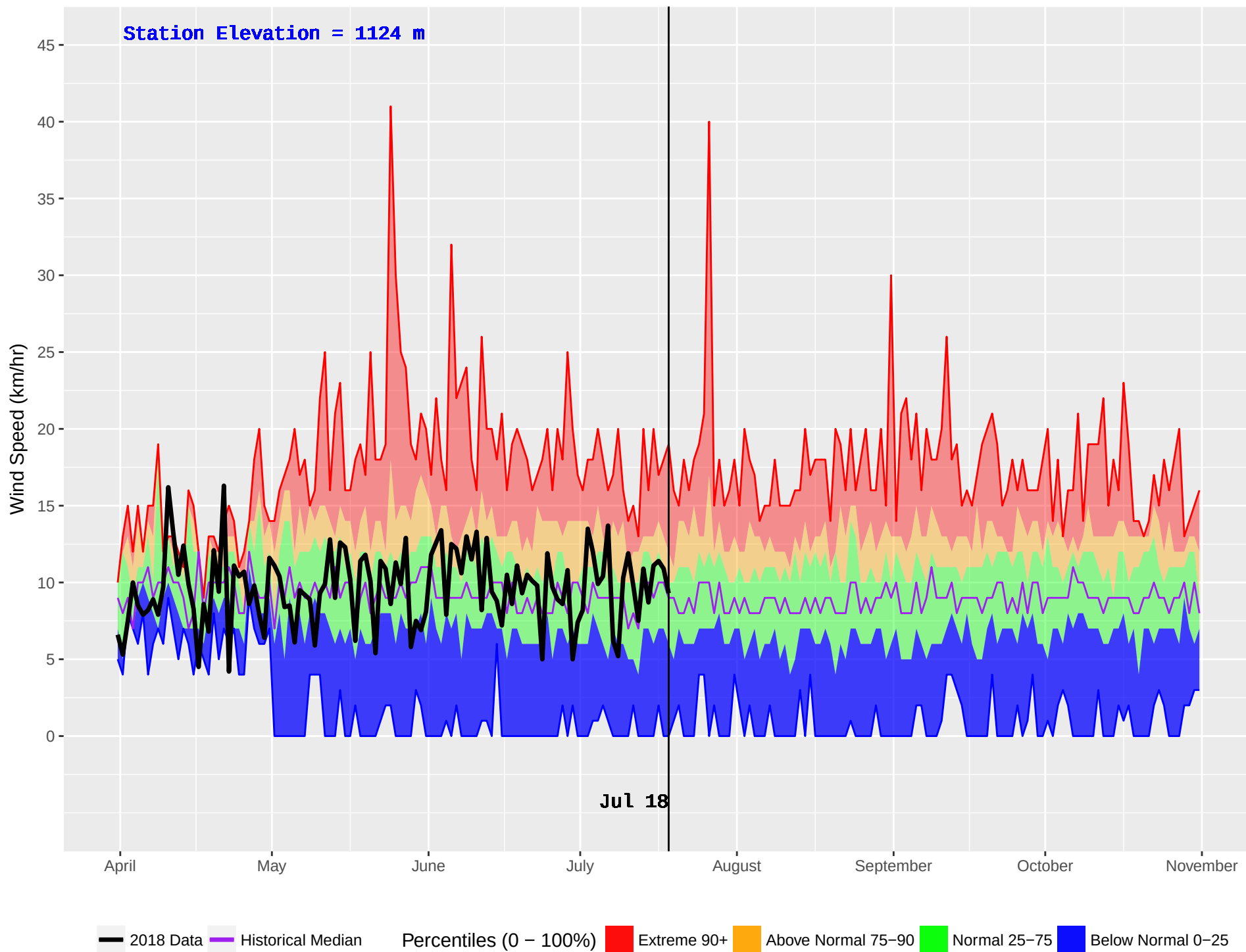
COLDSCAUR LAKE (232) : Historical (1979–2016) and Current (2018) Daily Wind Speed
