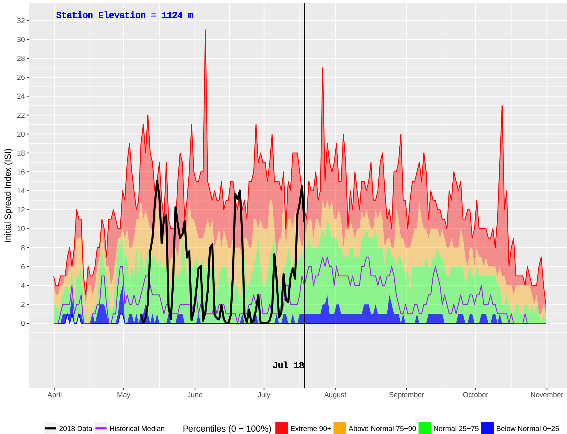
COLDSCAUR LAKE (232) : Historical (1979–2016) and Current (2018) Daily Initial Spread Index (ISI)
