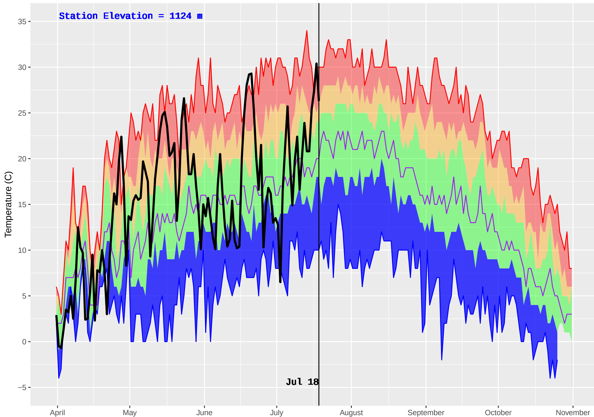
COLDSCAUR LAKE (232) : Historical (1979–2016) and Current (2018) Daily Temperature
